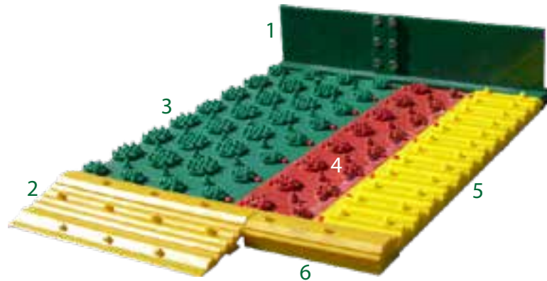
1) 4" Wall, 2) Transition border with berm, 3) Green Katch Mat™, 4) Red Katch Mat™, 5) Yellow Stab Mat, 6) 1" Berm
